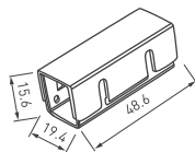
ARL-MOONLIGHT-1213- CON-POWER-MID-WH
