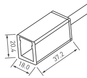
ARL-MOONLIGHT-1712- CON-POWER-HR-WH
