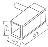
ARL-MOONLIGHT-1712- CON-POWER-RR-WH
