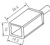
ARL-MOONLIGHT-1213- CON-POWER-HR-WH
