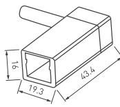
ARL-MOONLIGHT-1213- CON-POWER-RR-WH
